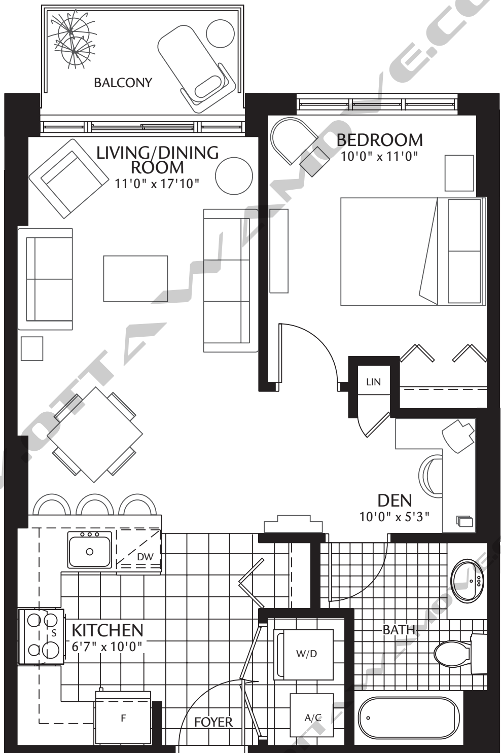
2ND FLOOR
